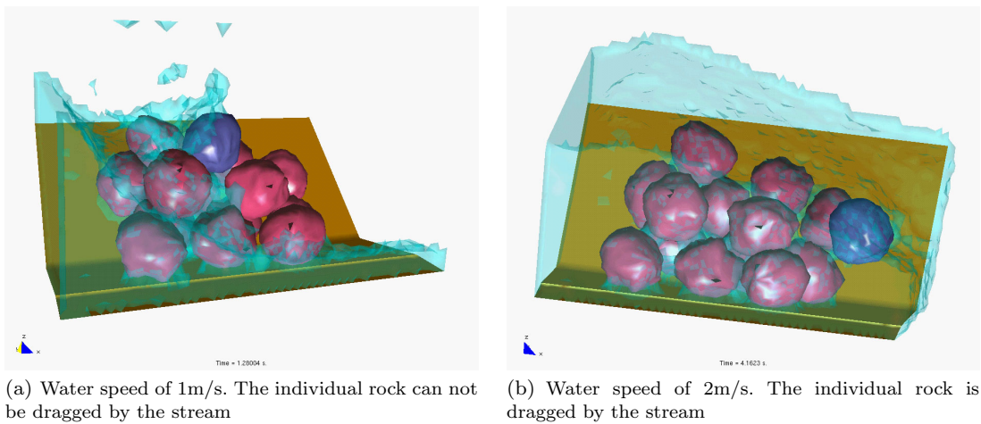
Fig. 4 Study of the drag of an individual rock of 1Tn under a water stream at speeds of a) 1m/s and b) 2m/s
