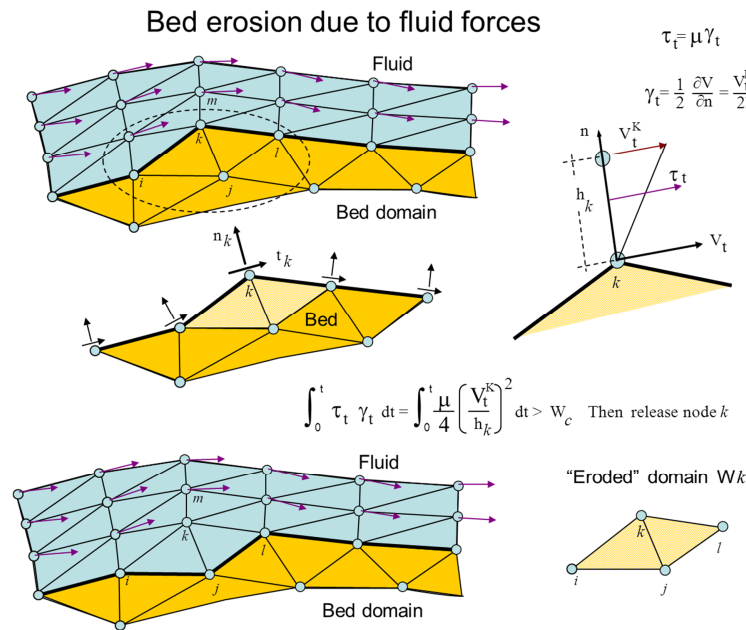
Fig. 3 Modeling of bed erosion with the PFEM by dragging of bed material
