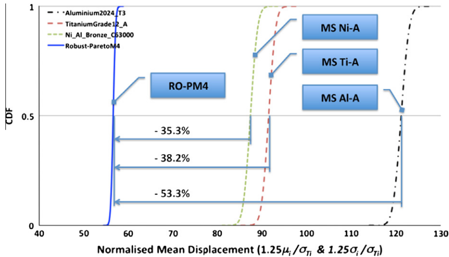
Fig. 13. Comparison of CDF obtained by MS Al-A, MS Ti-A, MS Ni-A and PM4 (Note: RO-PM i represents the i th robust optimal Pareto member).
